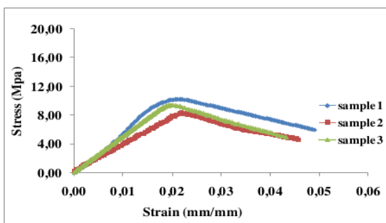
Fig 3. Stress – Strain Geopolymer Mortar Ratio 2.0 with The Percentage of Laterite Soil and Hydrated Lime 90; 10 ages 7 days
