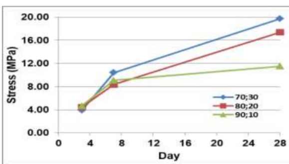
Fig 4. The Average Strength at aged 3, 7 and 28 days
